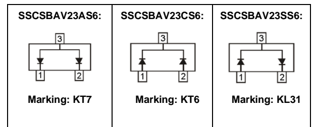
Circuit Diagram
